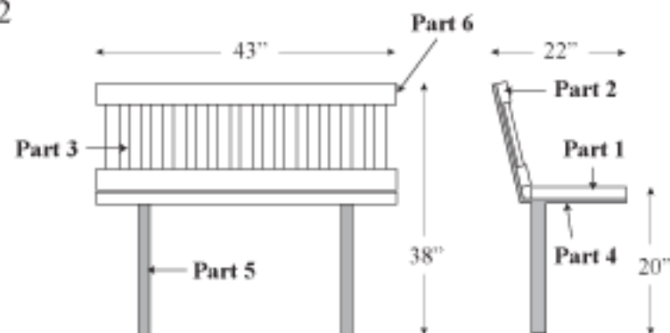
(Fig. 1) Product dimensions & Part identification.
