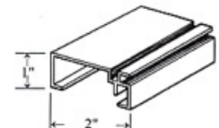
H121 - Horizontal supports...top, bottom and mullion
